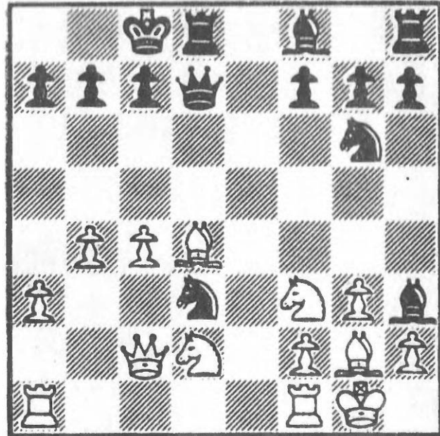
72 After 14 Bd4
